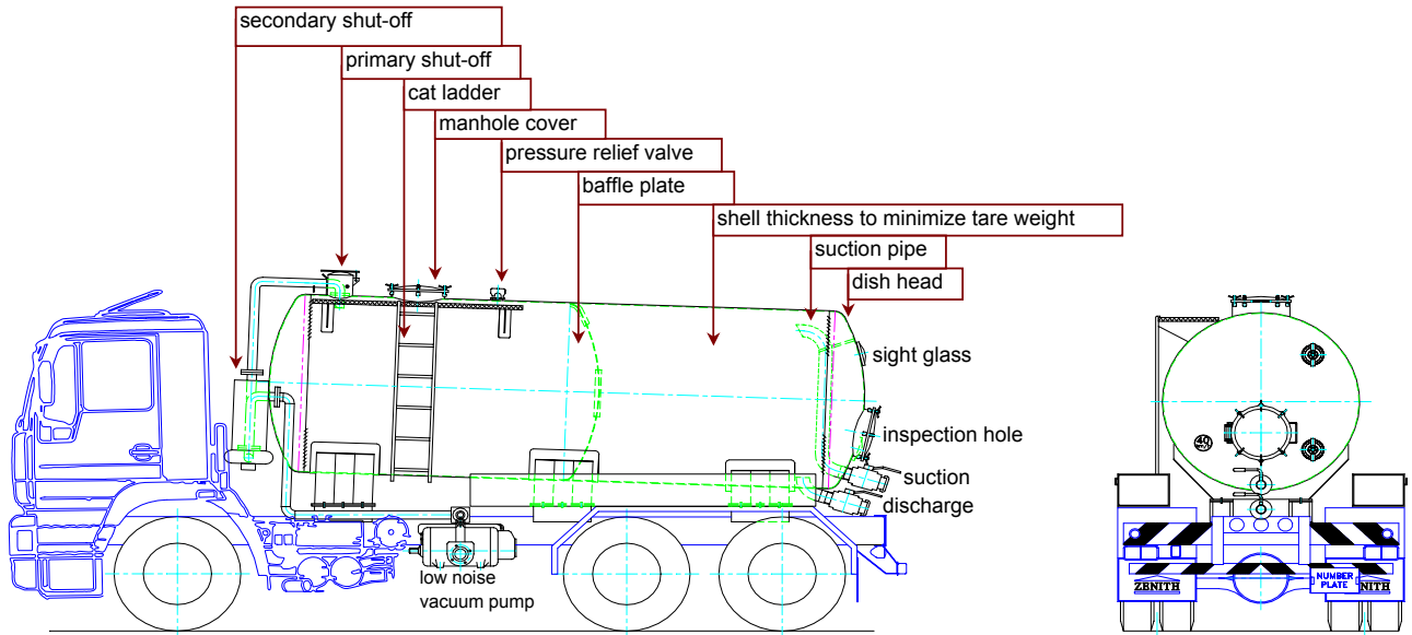
Basic configuration without tipping , hydraulic rear door , swivel boom nor hose reel .
